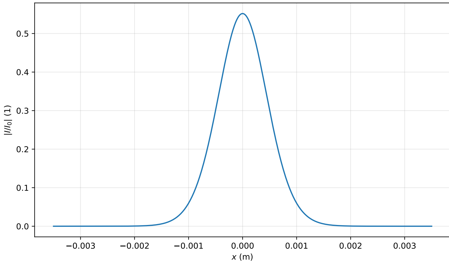
Intensity profile I(x, y = 0, z = 2.388m)/I_0 , P_{in}=0.3P_{cr} , artificial time
